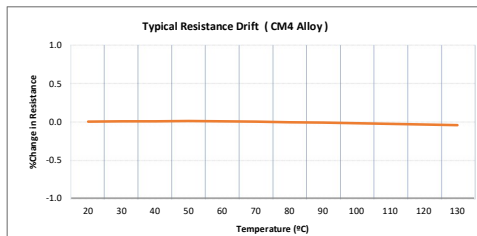
Resistance Change vs Temperature
